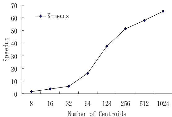
Fig. 8 Speedup under k
